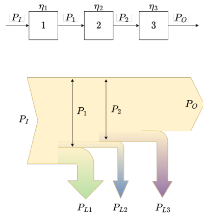
Fig. 23: Power flow diagram
