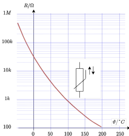
Fig. 19: NTC thermistor in the U-I-diagram
