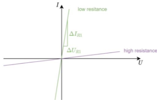
Fig. 13: Linear resistors in the U-I diagram
