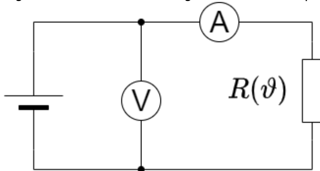
Fig. 16: Circuit for measuring the effect of temperature on a resistor
