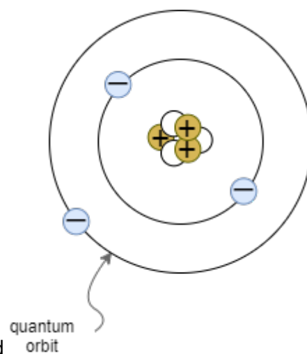
Fig. 1: Atomic model according to Bohr / Sommerfeld
