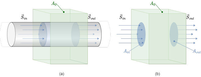
Fig. 5: Gauss's Law for Current Density
