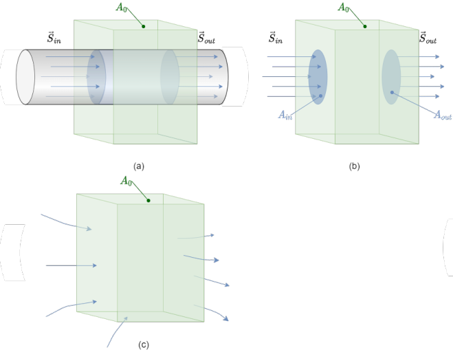
Fig. 5: Gauss's Law for Current Density
