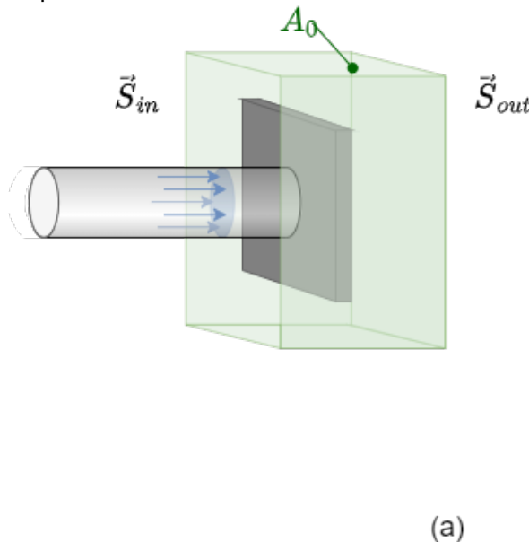
Fig. 6: Gauss's Law for Current Density for a Capacitor Plate
