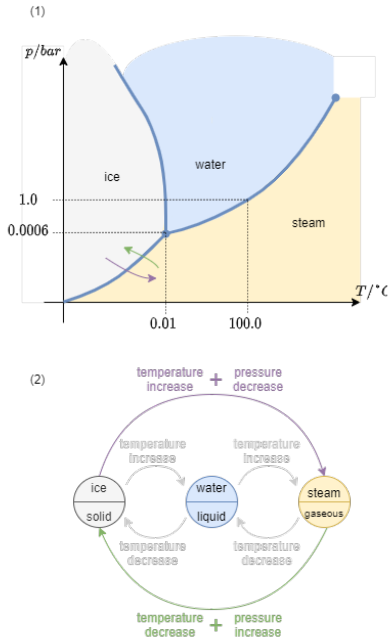
Fig. 10: State Diagram of water
